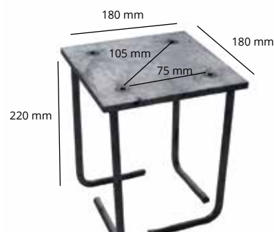
Ground anchor
