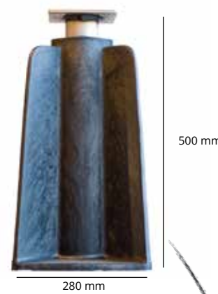
Inground base
